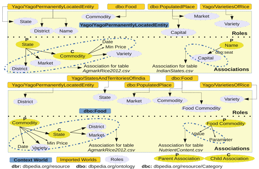
Fig. 3 Illustration of the working model of Many Worlds in a Frame (MWF) using open data tables
