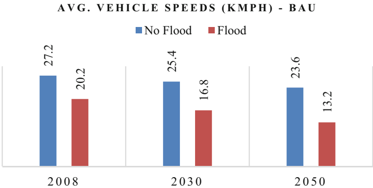
Fig. 17 Average vehicle speed comparison for flood and non-flood scenario
