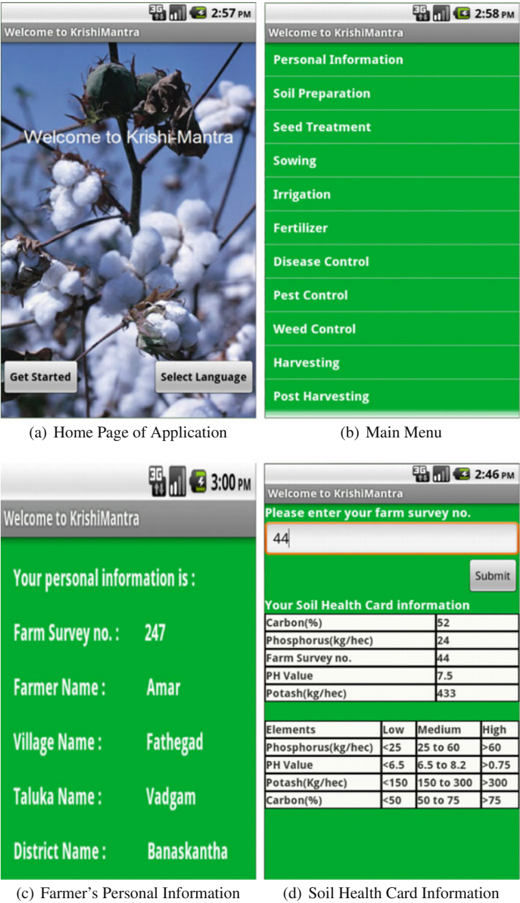
Fig. 4 Set of figures depicting the application interface
