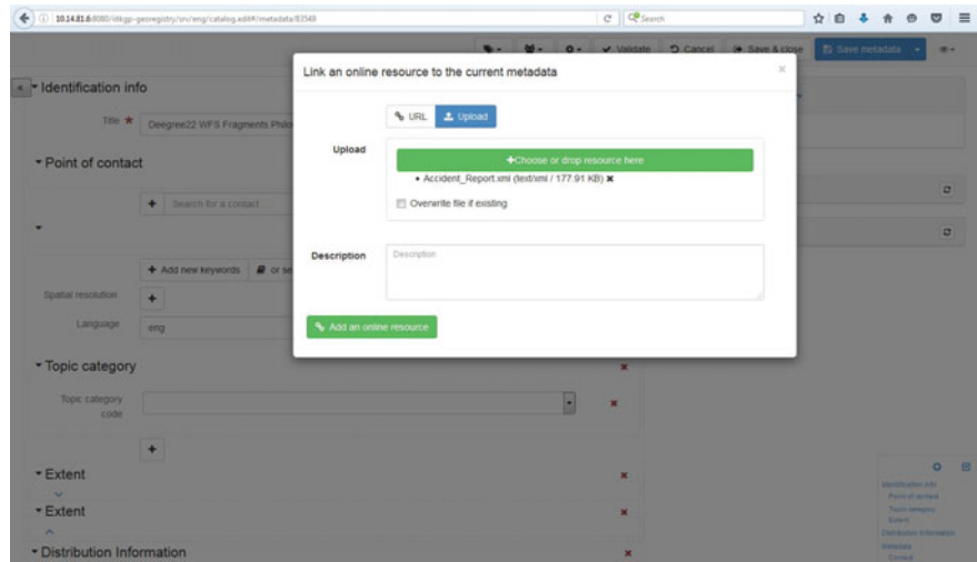
Fig. 6 Uploading ‘Accident_Report.xml’ file in spatial Web registry
