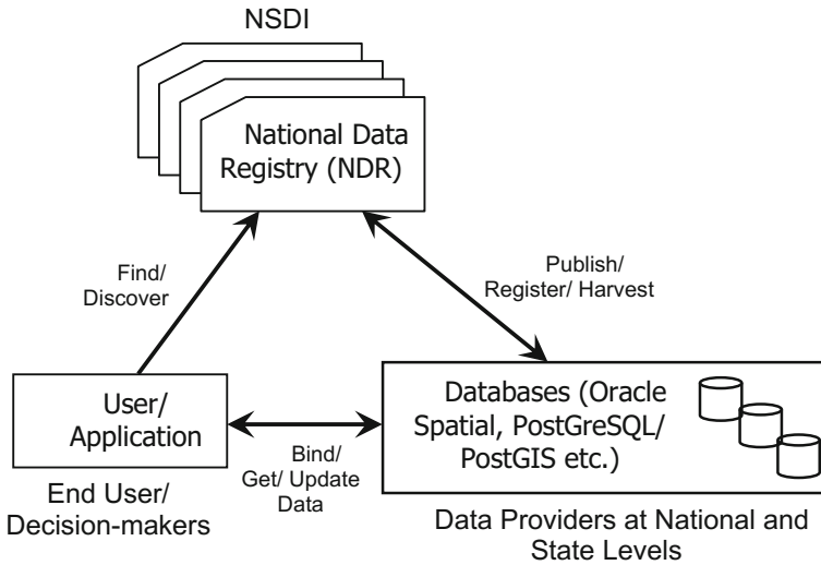
Fig. 1 Service-oriented architecture of NSDI-India—Publish-Find-Bind Model with National Data Registry
