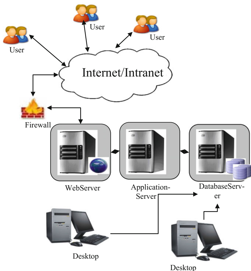
Fig. 1 Systematic representation of a common state's spatial database infrastructure (system architecture)
