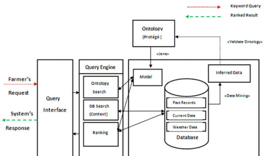
Fig. 1 OntoAQ architecture
