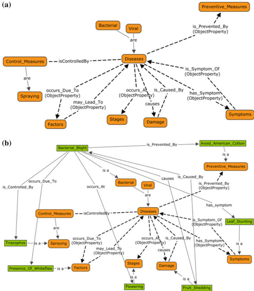
Fig. 2 a Crop ontology (generic) and b Cotton ontology (specific)
