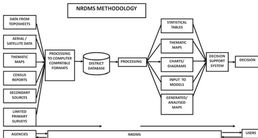
Fig. 1 NRDMS methodology
