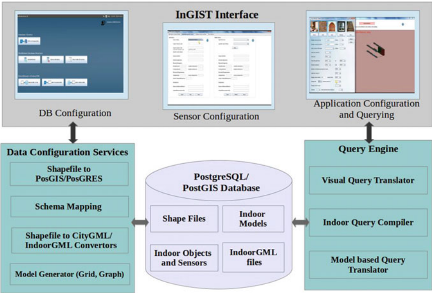
Fig. 2 InGIST architecture
